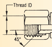
SAE 45° Flare Swivel Female (FSX)
