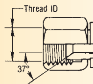
JIC 37° Flare Female (FJX)
